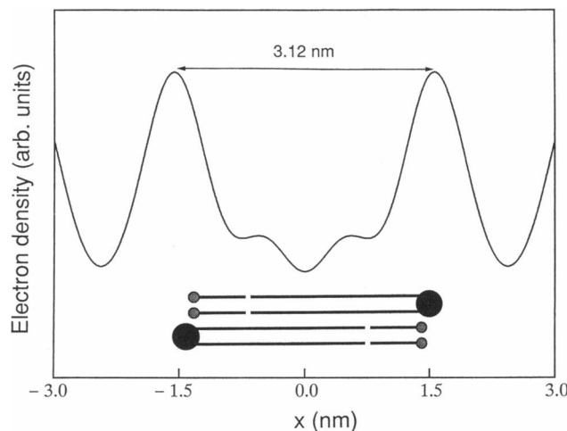
FIGURE 3 The one-dimensional electron density profile generated from the diffraction pattern given in Fig. 2. The adopted phases of the first to the fifth orders are (\pi, \pi, 0, \pi, \text{ and } \pi) (see text). A schematic view of the structure in the L_{\beta I} phase is inserted, with the black dots representing the lipid headgroups and the lines representing the lipid hydrocarbon chains.
